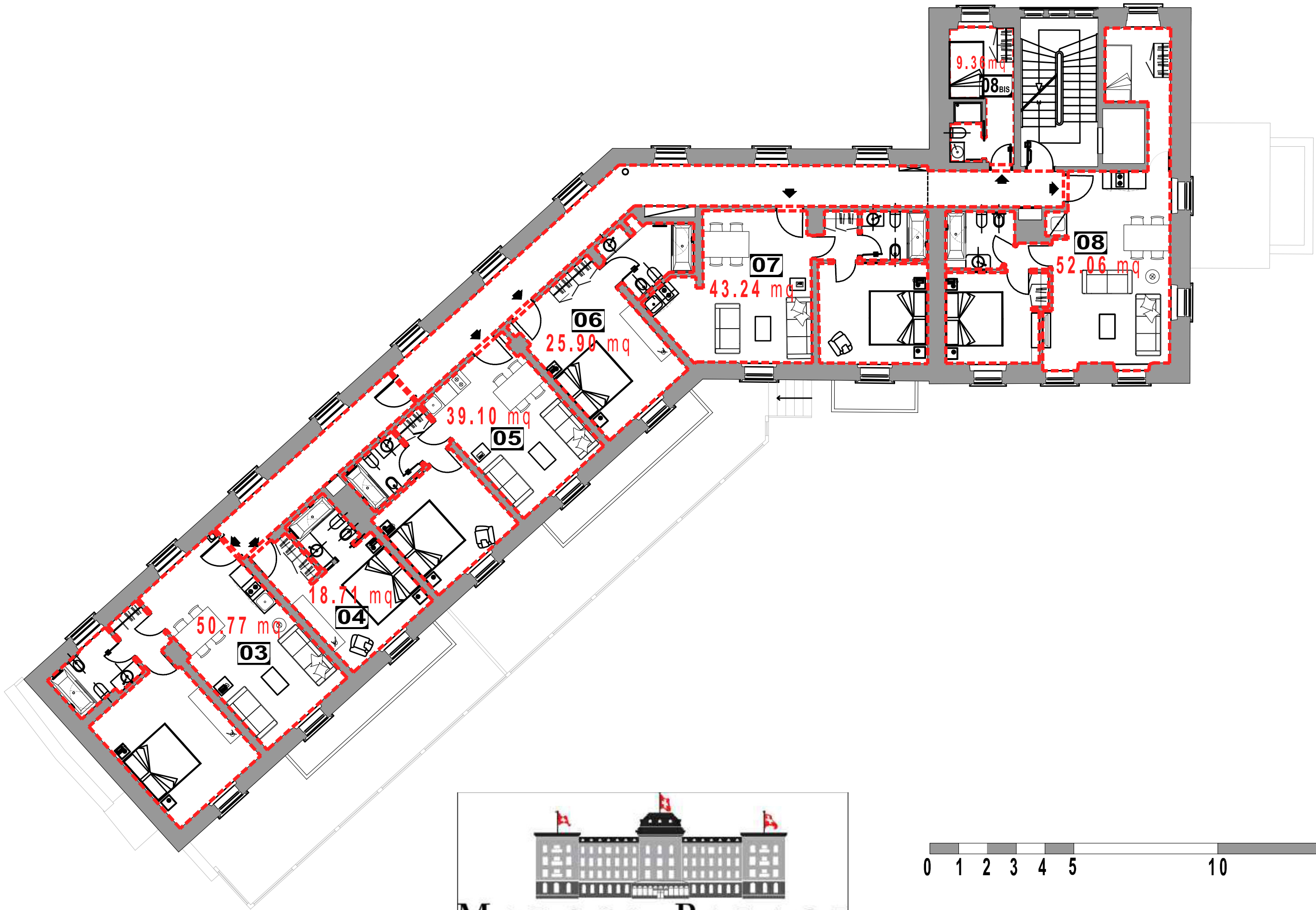
CLUB HOUSE GOLF - FIRST FLOOR
